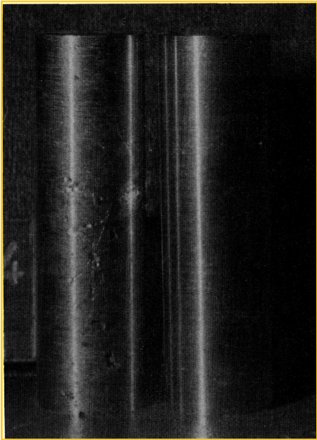
Fig. 4. Specimens of alloy 5 and alloy 6 after 7 days' immersion in 10% FeCl₃, pH 1.75, at 20°C, showing superior pitting resistance of alloy 5 (on R)
