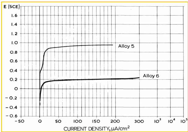
Fig. 3. Potentiostatic polarisation curves for alloys 5 and 6 in 3% NaCl (N₂-purged) at 30°C; N content of alloy 5 is 0.15% and of alloy 6, 0.05%
